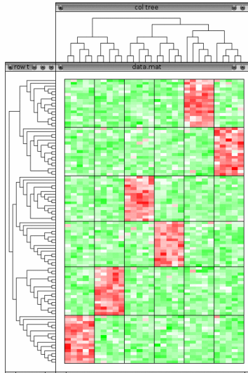
Figure 5: Example of row and column hierarchical trees in SUMMATRIX can be used to visualize a clustering. Cluster partitions (black horizontal and vertical lines) are shown with --rpart,cpart and trees are specified with --rptree,--cptree . See examples/summatrix/clustering/view_data_tree_clustered.sh
